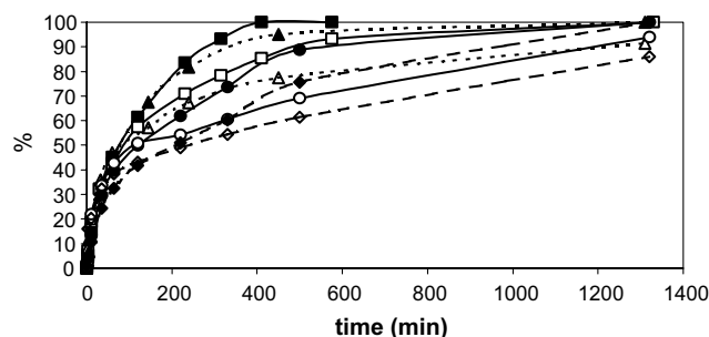
Figure 1. Analytical follow-up of the bihydrolysis of rac - 3 at 28 °C using StEH, under different experimental conditions: (a) H 2 O, DMSO (1%): ■ ee, □ conversion ratio; (b) Buffer, DMSO (1%): ▲ ee, △ conversion ratio; (c) H 2 O, DMF (1%): ● ee, ○ conversion ratio; (d) Buffer, DMF (1%): ◆ ee, ◇ conversion ratio.
